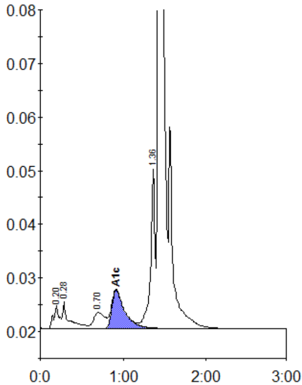
Peak table - ID: 10550955
